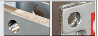
Pictured: Examples of the Drawer and the Rear Access Door Lock-Out
